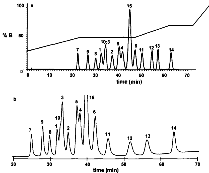
Fig. 4. Chromatogram of DRYLAB simulated (a) versus experimental (b) conditions using an optimized multi-segmented organic modifier gradient. (Gradient profile and other experimental conditions see Table 4; peak annotation see Table 1).
