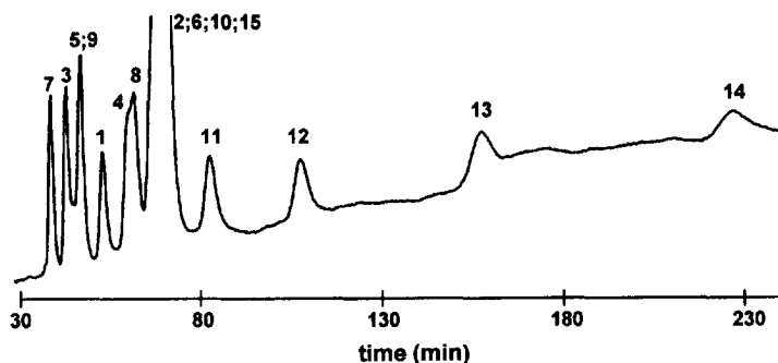
Fig. 2. Chromatogram of the initial experimental run. (Peak annotation and chromatographic conditions see Table 1).
