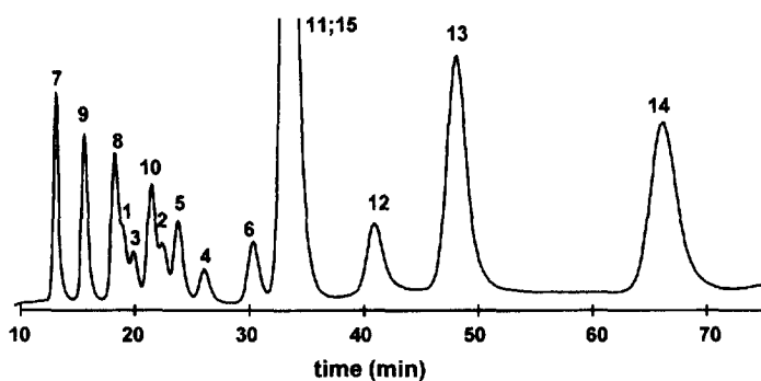
Fig. 3. Chromatogram at optimized experimental and isocratic conditions. (Mobile phase: 110 mM ammonium acetate-(ACN-THF, 99:1), (55:45, v/v); pH a 5.5; T=25°C; peak annotation see Table 1). The given molarity value refers to that of the final mixture.
