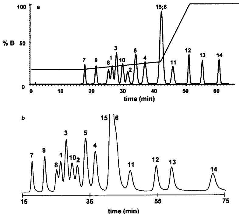
Fig. 5. Chromatogram of DRYLAB simulated (a) versus experimental (b) conditions using an optimized multi-segmented buffer salt gradient. (Gradient profile and other experimental conditions see Table 5; peak annotation see Table 1).
